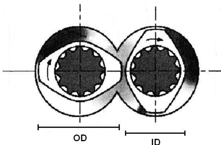
Fig. 60 Ratio of outside and inside diameter (OD/ID) of a screw, modified according to Thiele (2003)
