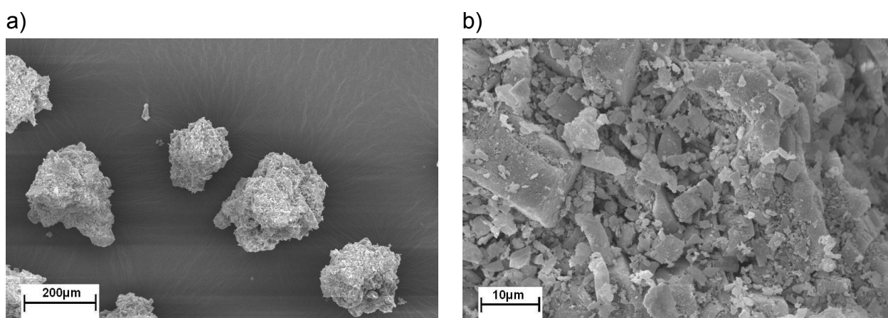
Fig. 57 Micrographs of dicalcium phosphate particles at different magnifications
