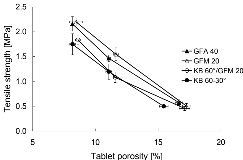
Fig. 25 Tensile strength of mannitol tablets for different screw configurations (n=10, mean±s)
