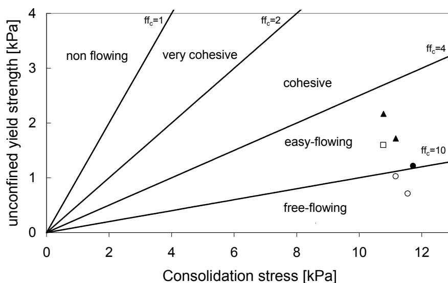
Fig. 45 Flowability of different dicalcium phosphate granules ( n=3 ) (▲ = Conveying elements, □ = Combing mixer elements, ○ = Kneading blocks, ● = Kneading block / Combing mixer element combination)
