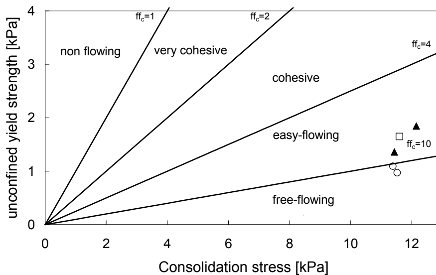
Fig. 30 Flowability of different dicalcium phosphate granules ( n=3 )
