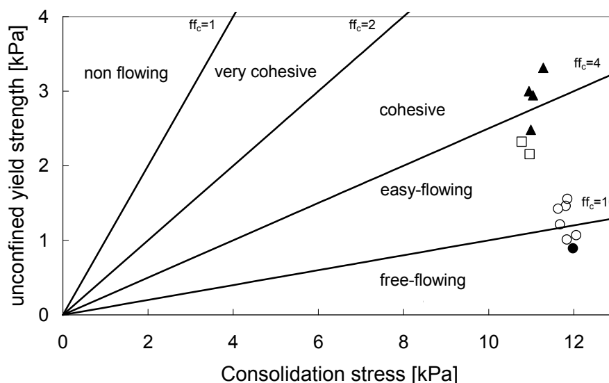
Fig. 24 Flowability of different mannitol granules (n=3) (▲ = Conveying elements, □ = Combing mixer elements, ○ = Kneading blocks, ● = Kneading block / Combing mixer element combination)
