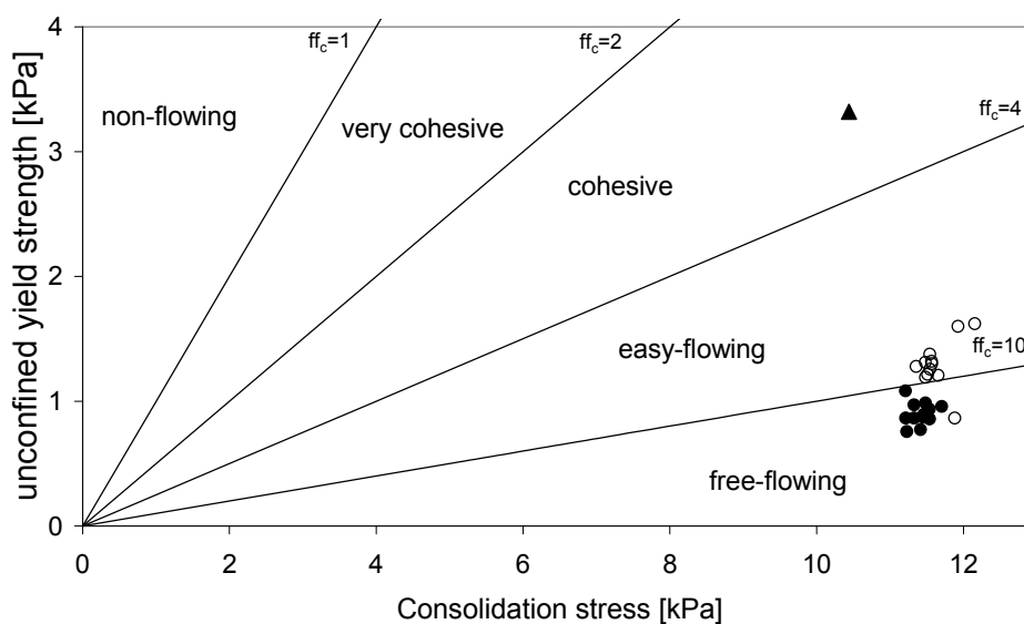
Fig. 68 Flowability of lactose granules (n=2), ● = APV extruder, ○ = Leistritz extruder, ▲ = initial powder
