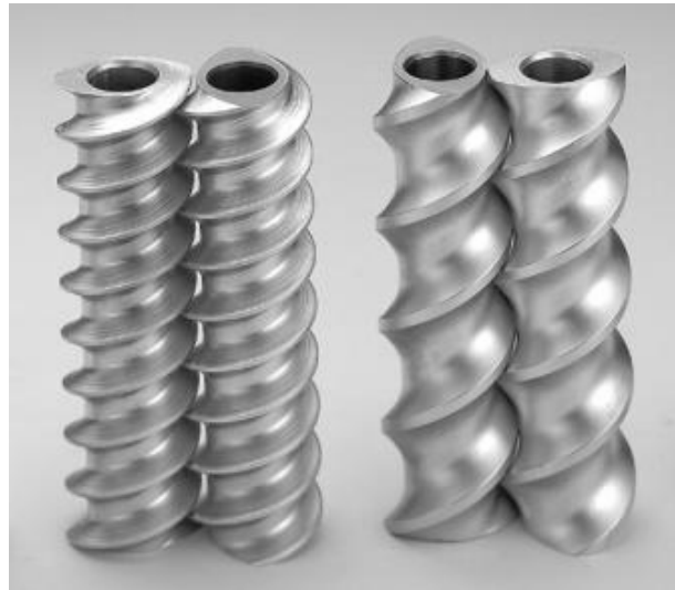
Fig. 1 Conveying elements of 90mm length with 20mm element pitch (left) and 40mm pitch (right)
