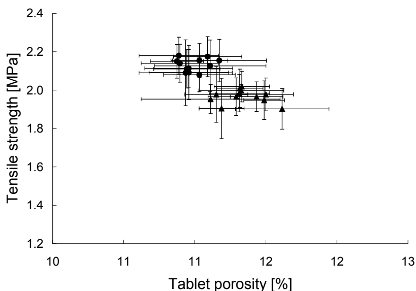
Fig. 69 Tablet tensile strength of lactose tablets (n=10, mean \pm s) (● = APV extruder, ▲ = Leistritz extruder)
