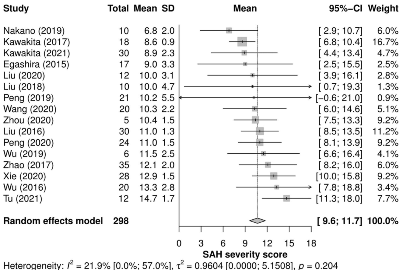
Fig. 5 SAH severity grade forest plot. Random-effects meta-analysis. The column “Total” shows the number of mice per article subjected to SAH grading. The column “Mean” represents the SAH severity
