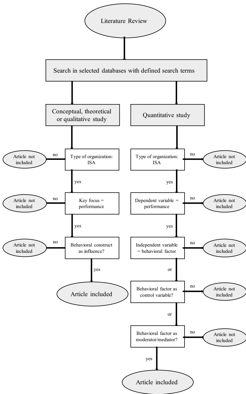
Fig. 5 Decision tree
