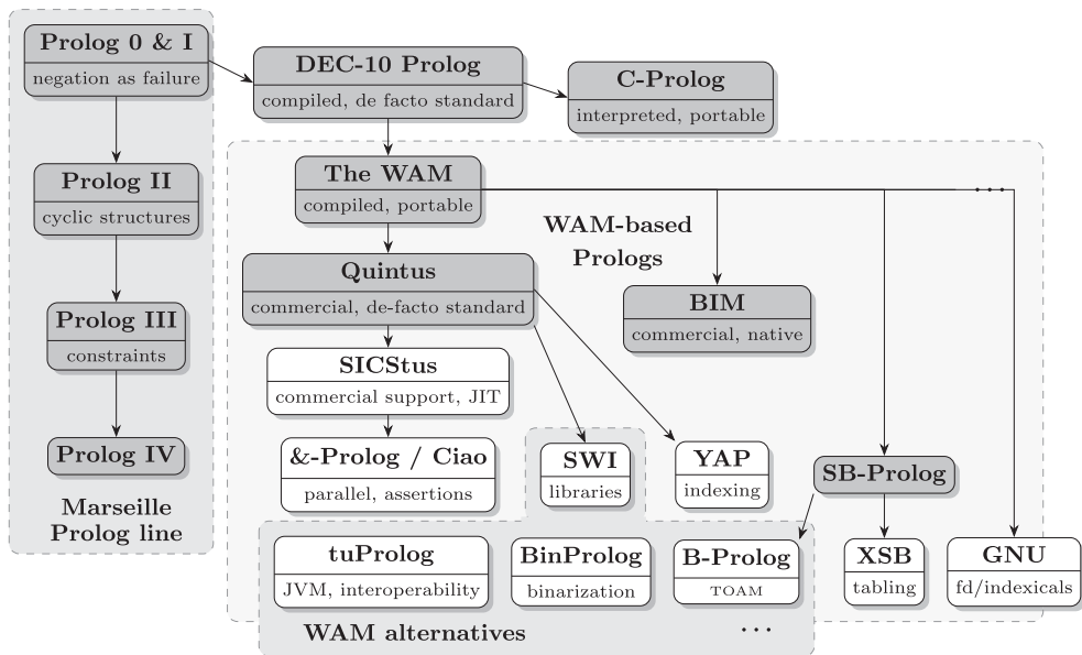
Fig. 2. Prolog Heritage. Systems with a dark gray background are not supported any more. Arrows denote influences and inspiration of systems. The bottom section of each block includes just some highlight(s); see the text for more details. Quick legend: JIT = “Just in Time [Compiler]”, JVM = “Java Virtual Machine”, TOAM = “Tree-Oriented Abstract Machine”.
