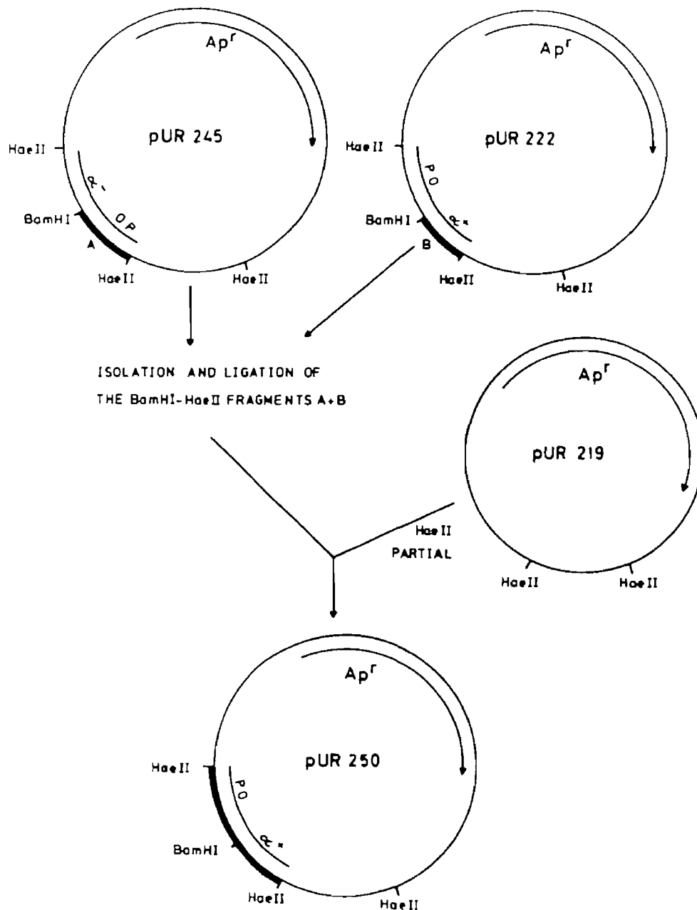
Fig. 2 Construction of plasmid pUR 250. The combined polylinker regions of plasmids pUR 245 and pUR 222 contain all desired restriction sites and allow the expression of an active \alpha - peptide of the lac Z gene. Therefore the Bam HI - Hae II fragments A and B of these plasmids were isolated and ligated. After recutting with Hae II these fragments were cloned into the partially Hae II digested plasmid pUR 219. This plasmid is identical to pUR 222 but does not contain the Hae II fragment carrying the lac promoter, operator and the beginning of the lac Z gene which codes for the \alpha - peptide. As a result plasmid pUR 250 was obtained.
